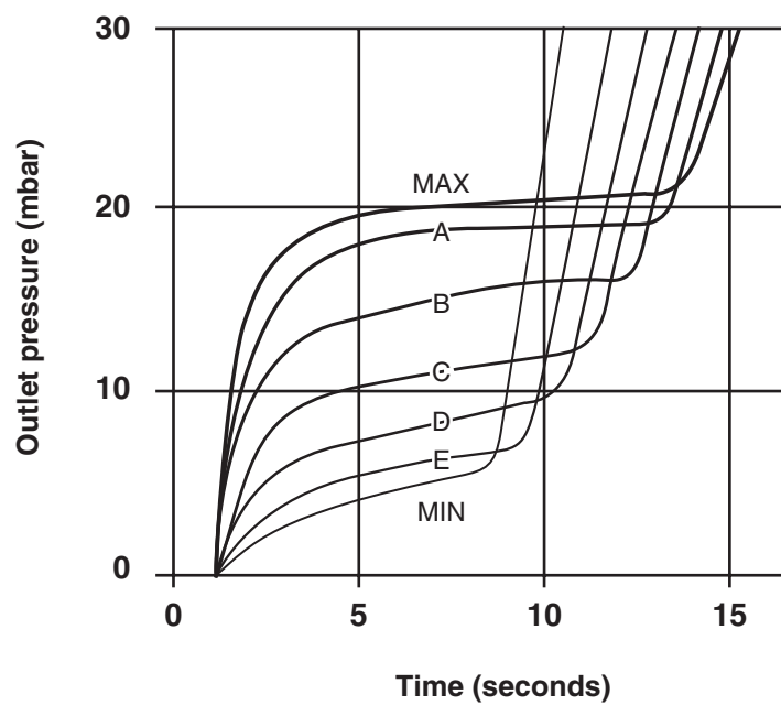
Fig. 18. Adjustable SOFTLITE
